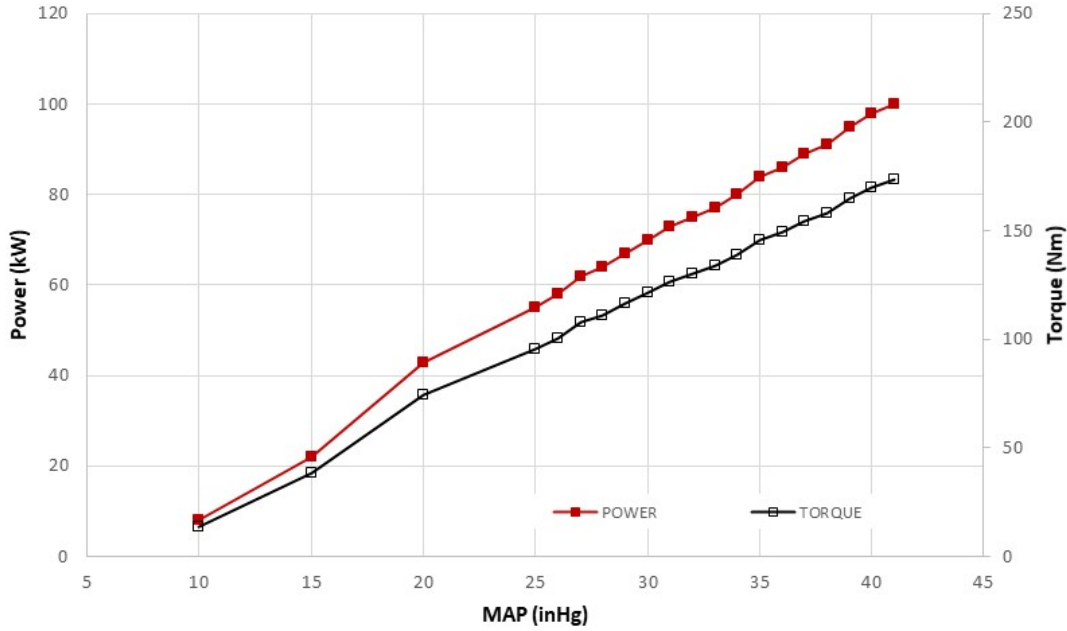
ENGINE PERFORMANCE @5500 RPM
