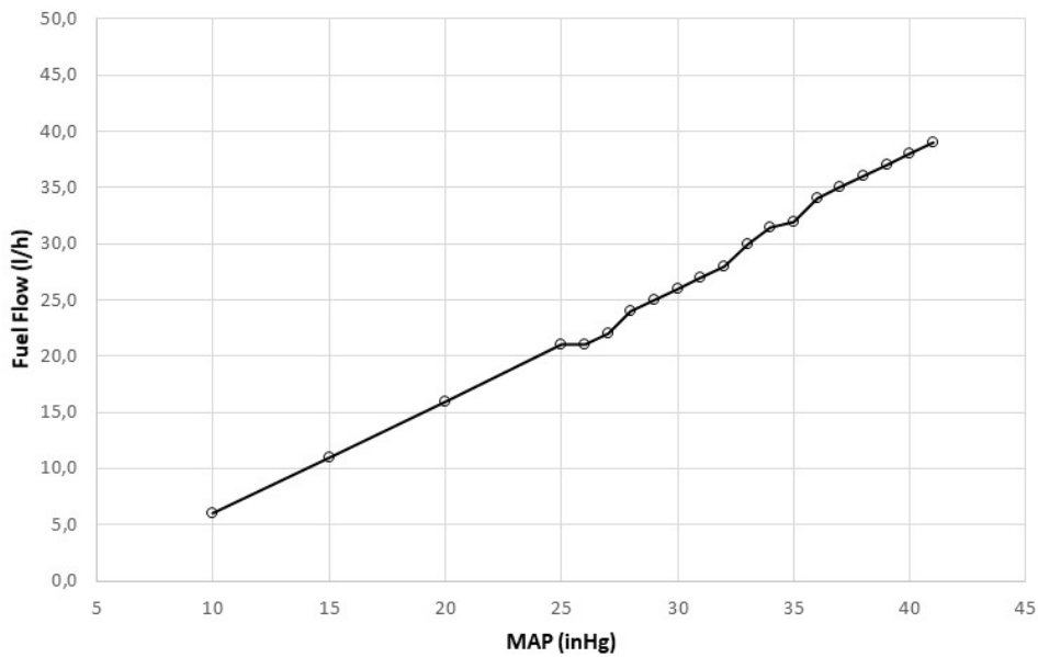
FUEL FLOW @5500 RPM
